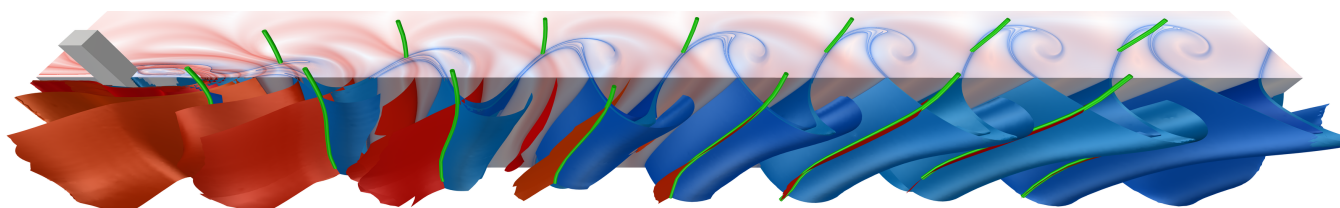
Figure 1: Time-dependent vector field topology of the von Kármán Vortex Street dataset at t=0.5 s, defined by attracting/repelling Lagrangian coherent structures (LCS, blue/red surfaces), obtained as streak manifolds seeded along hyperbolic path surfaces (time slice by green lines). Our local extraction yields a geometric representation of the temporal evolution of the LCS, which is consistent with ridges in the backward- (blue) and forward-time (red) FTLE fields. Sections of the FTLE fields shown in the back half, streak manifolds clipped at the top for clarity.
