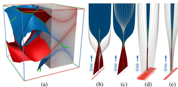
Figure 8: (a) ABC Flow: while traditional VFT is empty, bifurcation lines (green) and their invariant manifolds (red/blue) capture the separating behavior of the flow consistently with the FTLE. (b)–(e) Scale-dependency of the FTLE (red, bottom). Strongly separating LCS (b) appears weak at smaller scales (c). Weakly separating LCS (d) appears strong at larger scales (e). Hyperbolic trajectory (green) and attracting/repelling streak manifolds (blue/red).
