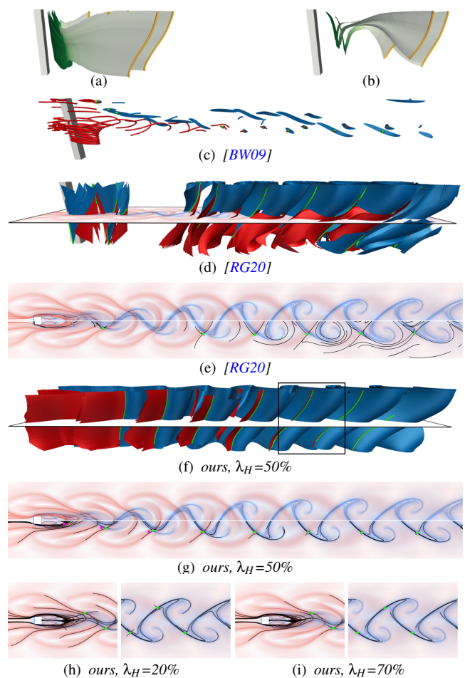
Figure 11: Backward-time integration along observer motion \mathbf{f}(\mathbf{x}, t) for Galilean-invariant (a) and displacement-based (b) optimal frames of reference started on bifurcation lines in \mathbf{w}(\mathbf{x}, t_0) . Considering saddle-type critical points in \mathbf{w} as initial candidates for hyperbolic trajectories, i.e., a straightforward extension of the 2D method [HS20], misses most of the topological structure (c), while vector field topology in an optimal steady reference frame is not aligned with LCS (d),(e). Computed from a Galilean-invariant frame of reference, our method captures large parts of the topology, and is aligned with LCS (f),(g). Green: saddle points and bifurcation lines, blue/red: attracting/repelling LCS. Raw features shown in magenta in (g). (e) and (g) show cross-sections from (d) and (f), with manifolds slices shown in black. (g)–(i) Streak manifolds with seeding lengths (Section 4.3.2) from different percentages of FTLE.
